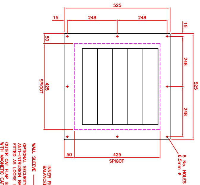
END VIEW (INTAKE)
